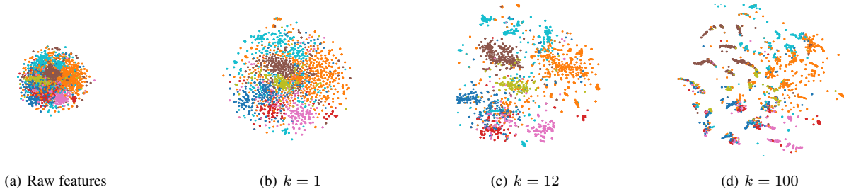
Fig. 3: (a-d) t-SNE visualization of the raw and filtered node features of Cora with different k .
