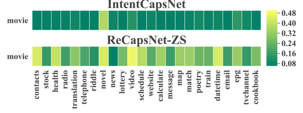
Figure 3: Comparison of the similarity scores between the unseen intent “movie” and the seen intents learned by IntentCapsNet and ReCapsNet-ZS (ours).
